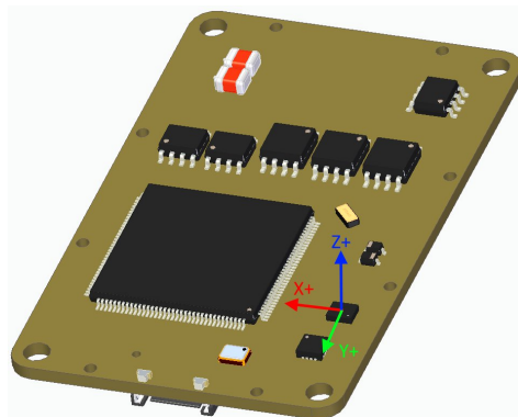
Figure 3-9: Gyroscope &amp; accelerometer coordinate system
