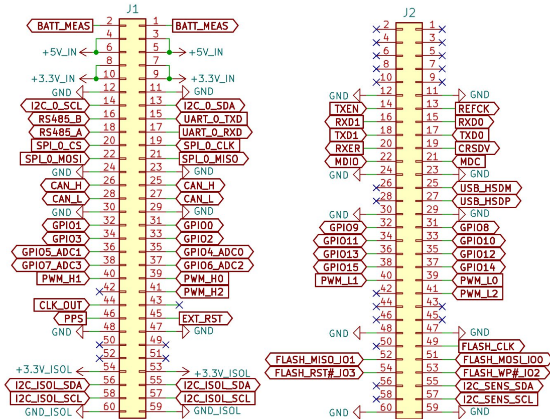
Figure 3-2: Main connectors (J1 & J2)
