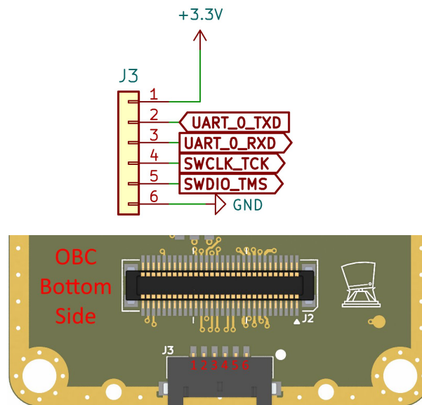
Figure 3-1: Programming connector
