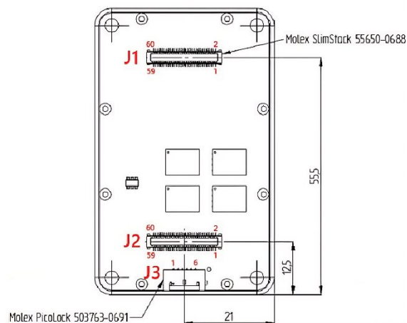
Figure 3-3: Connector pin numbering
