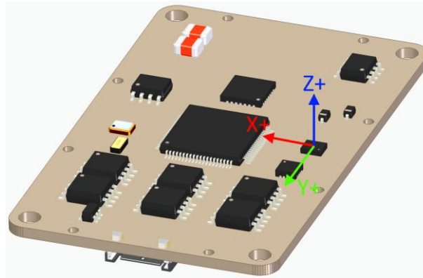
Figure 3-7: Gyroscope & accelerometer coordinate system
